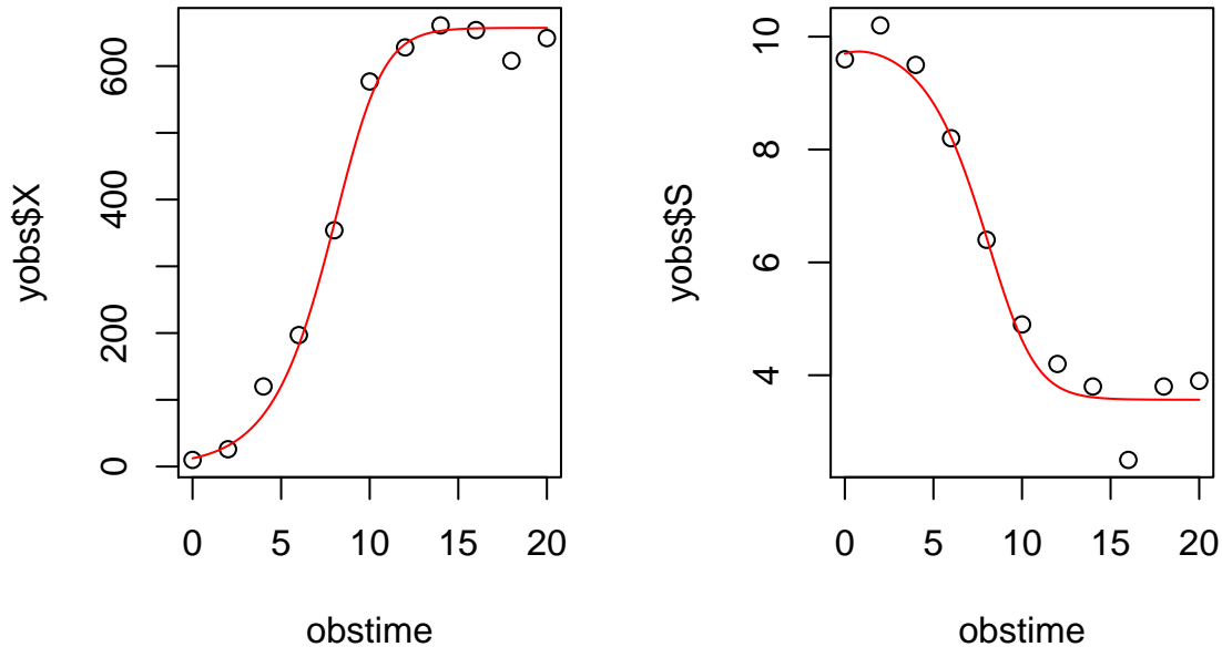
Figure 6: Observed data and fitted model ( k_m , v_m and initial values were estimated).
