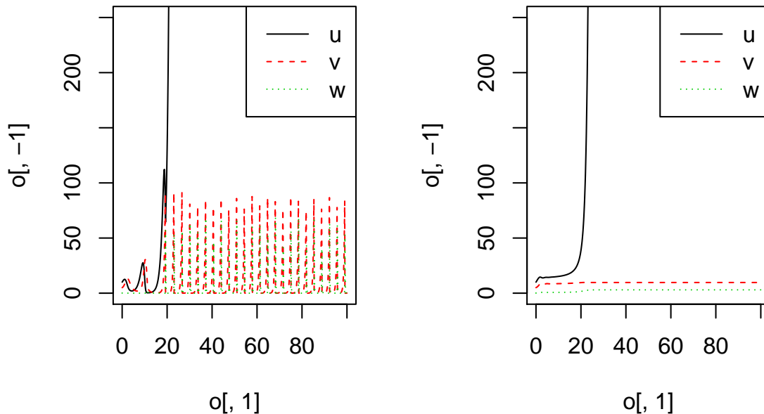
Figure 2: Two scenarios of the UPCA model (left: w_{star}=0 , right: w_{star}=0.1 ; functional response f is Holling II).
